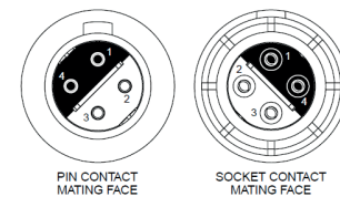
Suggested Numbering for Quadrax Contacts
