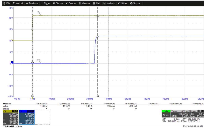
Start-up Waveform Vin = 110V, 0A Load
