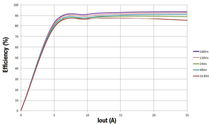
Power Efficiency vs Load
