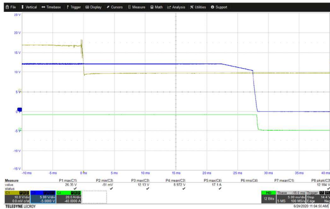
Hold Up/Interruption Time: Measured hold up time with 12Vo/200W Ch1: Vin Ch3: Vout Ch4: Iout (NOTE: for models with Hold Up option)
