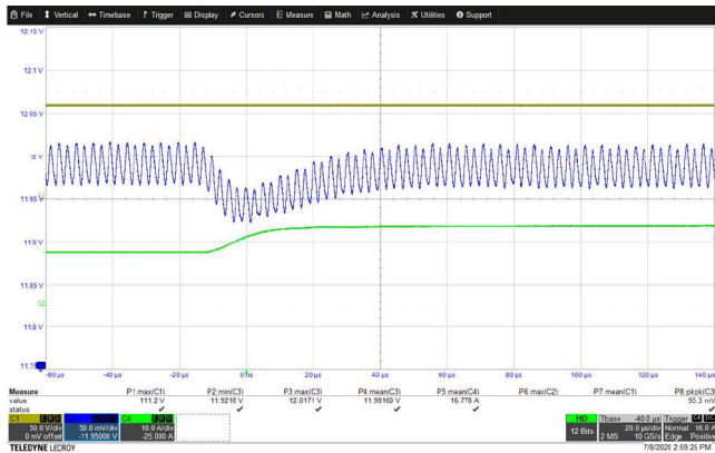
Transient Response Vin = 110V (Ch1), Vout (Ch3), Iout (Ch4) Step Load 50% → 75%, 20us/div. Vpp=96mV
