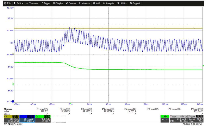
Transient Response Vin = 110V (Ch1), Vout (Ch3), Iout (Ch4) Step Load 75% → 50%, 20us/div. Vpp=103mV
