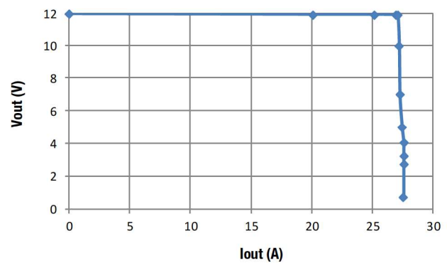
Overload Protection at Vin = 110V @ 22°C
