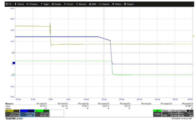
Hold Up/Interruption Time: Measured hold up time with 12Vo/300W Ch1: Vin Ch3: Vout Ch4: Iout (NOTE: for models with Hold Up option)
