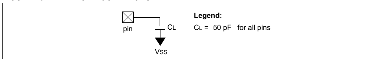
FIGURE 10-2: LOAD CONDITIONS
