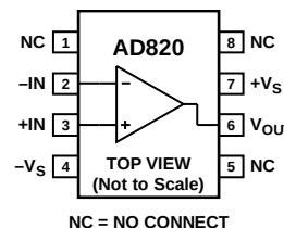
Figure 2. 8-Lead SOIC_N and 8-Lead MSOP
