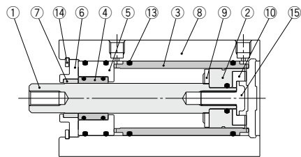
Lateral load resisting type: MQQL (Built-in ball bushing)
