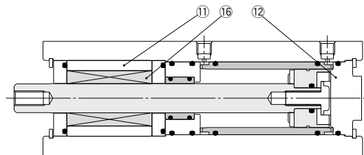
Lateral load resisting type: MQQL (Built-in ball bushing)
