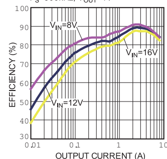
Efficiency vs. Output Current F_s=500\text{kHz} , V_{OUT}=1\text{V}
