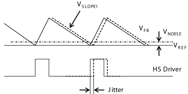
Figure 4: PWM-Mode Jitter
