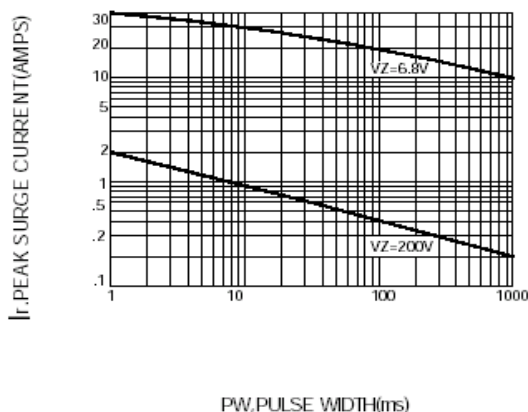
FIG. 2 - PEAK SURGE CURRENT VS PULSE WIDTH
