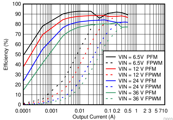
Figure 9-12. Efficiency
