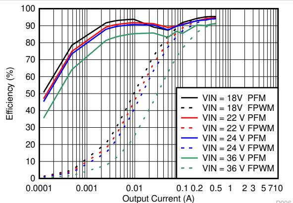
Figure 9-24. Efficiency
