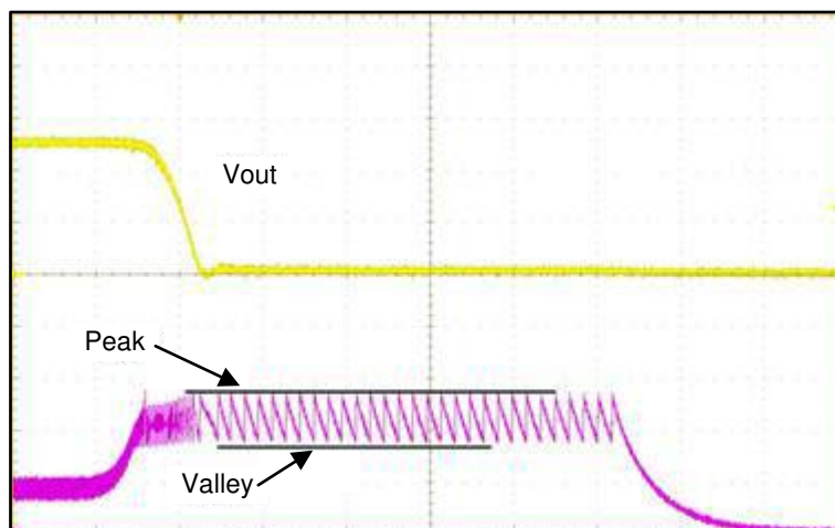
Figure 8-1. Current Limit Operation During Output Short Circuit
