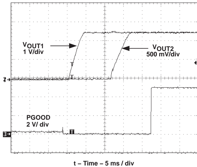
Figure 18. Simultaneous Startup
