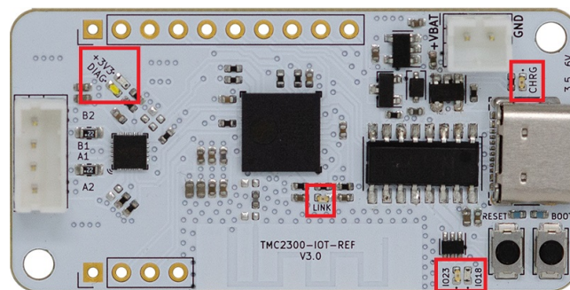
Figure 2: TMC2300-IOT-REF Onboard LEDs
