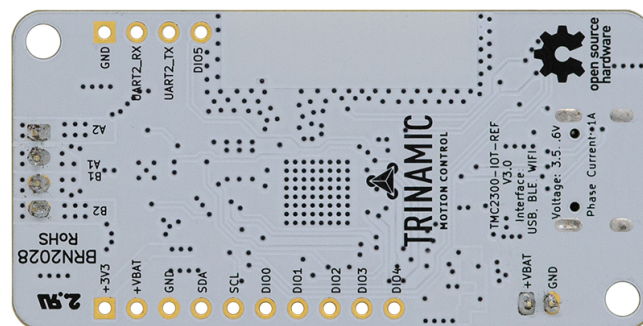
Figure 1: Bottom side of the TMC2300-IOT-REF board
