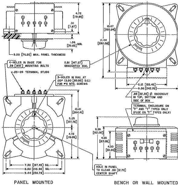
PANEL MOUNTED
