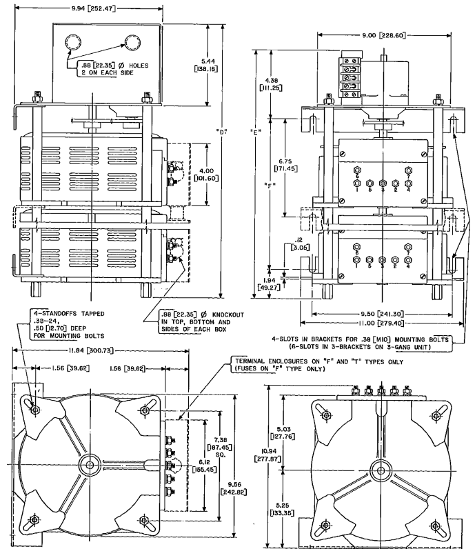
MOTOR DRIVEN
