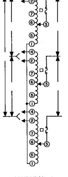
CONNECTION 4
