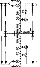
CONNECTION 2
