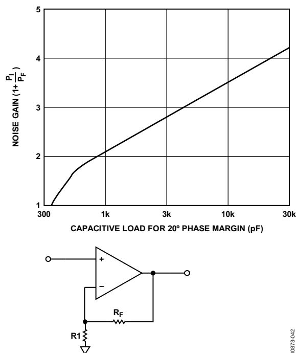
Figure 41. Noise Gain vs. Capacitive Load Tolerance
