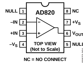
Figure 1. 8-Lead PDIP
