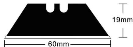
Lame de rechange 41-1311.704
