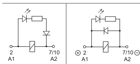
C: Varianti 3, 5, 54 LED (AC)
