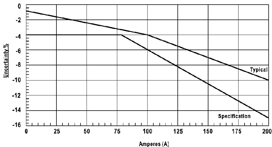
Figure 8: DC signal linearity in the 10 mV/A range, typical
