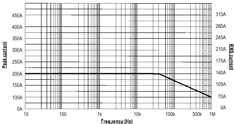
Figure 7: Maximum current versus frequency
