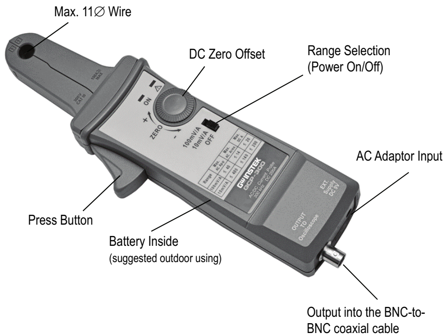
Figure 1: shows the controls and indicators on the GCP-300 current probe.
