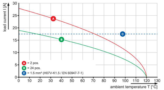
LSF-SMT 3.81/./90 3.5
