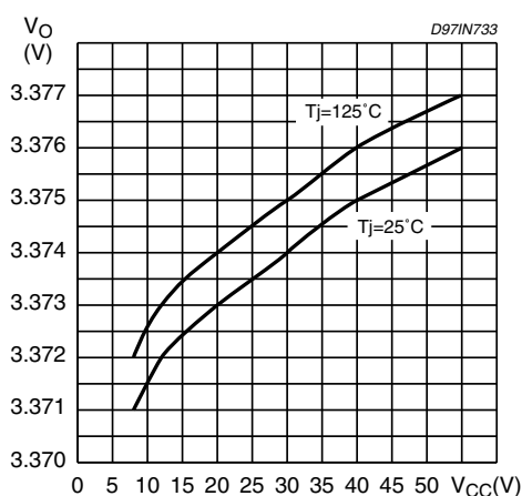
Figure 10. Load regulation
