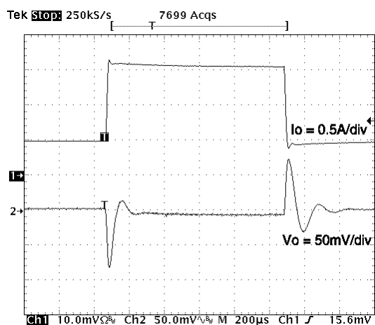
Figure 25. Line transient.
