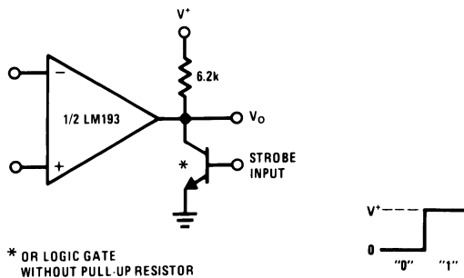
Output Strobing
