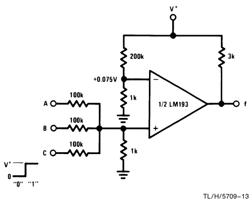
OR Gate
