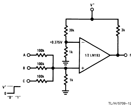
AND Gate
