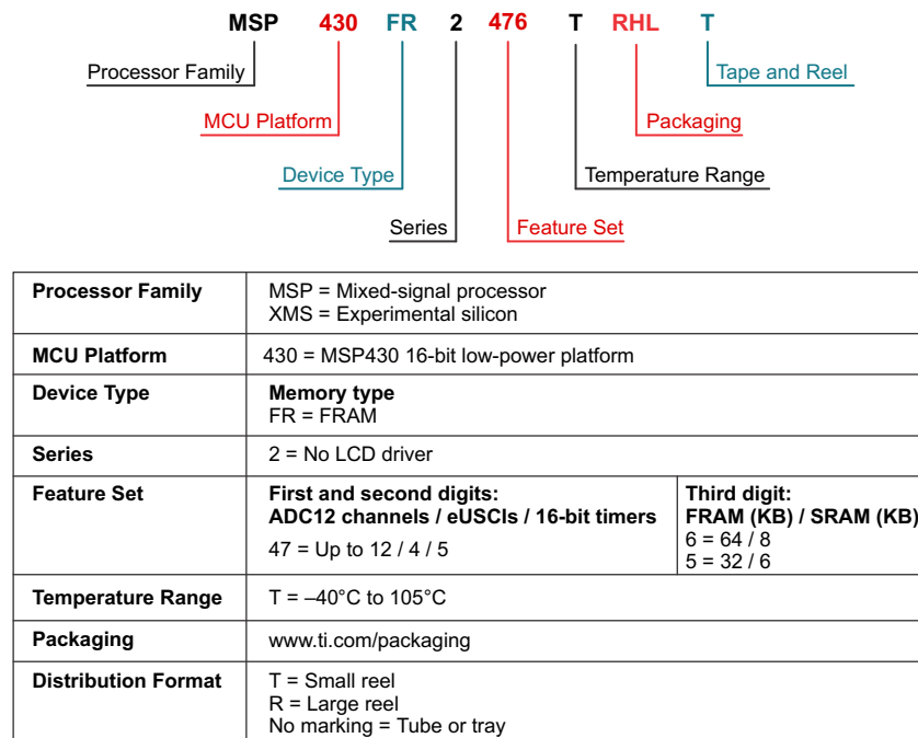
Figure 11-1. Device Nomenclature
