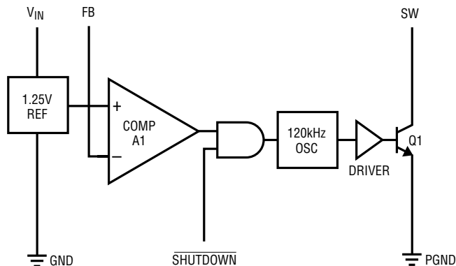
LT1109A (Adjustable)
