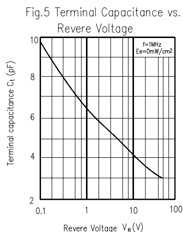
Fig.5 Terminal Capacitance vs. Reverse Voltage
