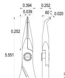
Dimensions in inch
