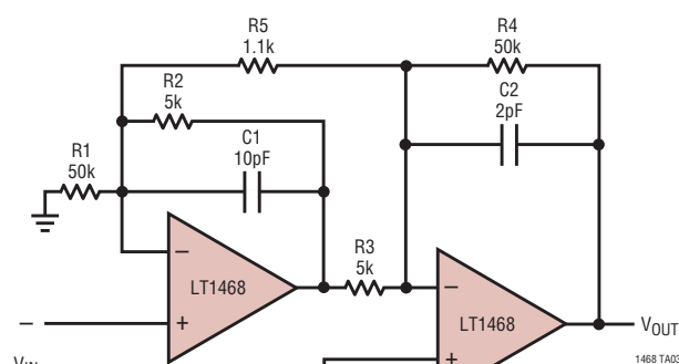
Instrumentation Amplifier
