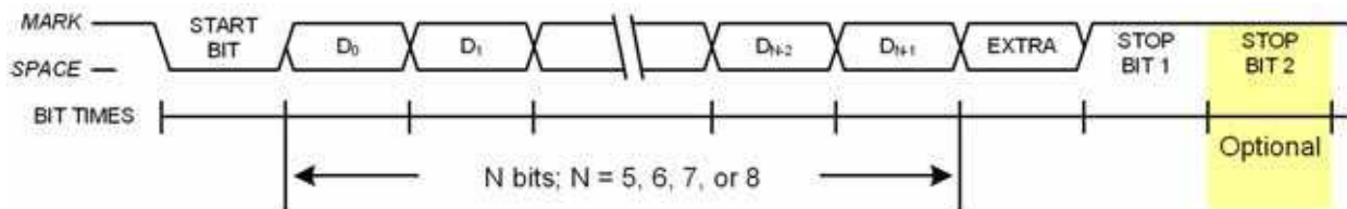
Figure 23.4. UART1 Timing With Extra Bit
