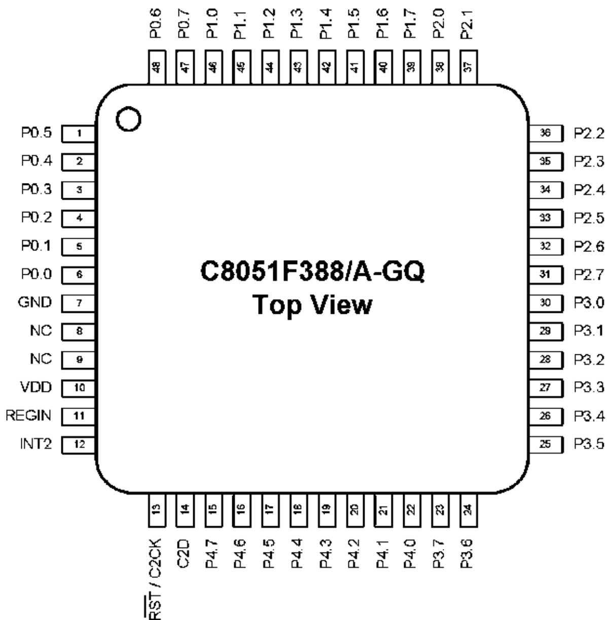
Figure 3.1. TQFP-48 (C8051F388/A) Pinout Diagram (Top View)
