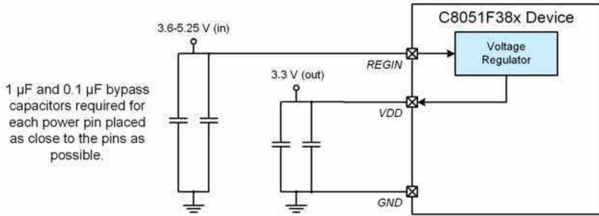
Figure 4.1. Connection Diagram with Voltage Regulator Used
