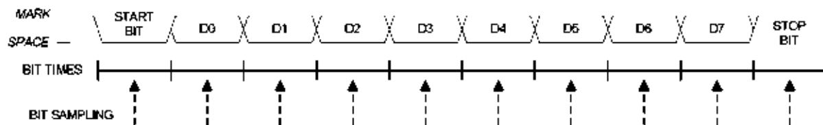
Figure 22.4. 8-Bit UART Timing Diagram
