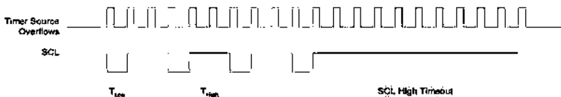
Figure 21.4. Typical SMBus SCL Generation
