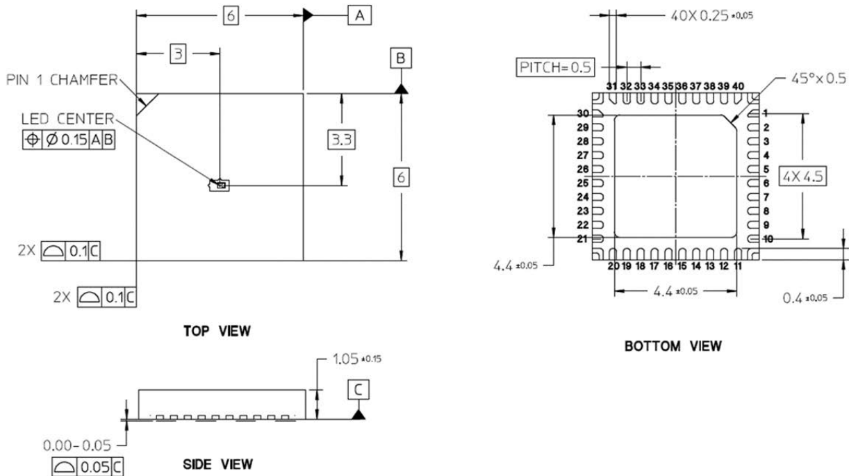
Figure 5: Overall Package Dimension and Pinout
