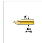
POGO-25T36-S
