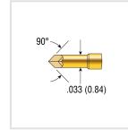
POGO-25T36
