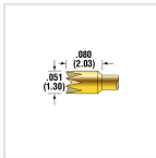
POGO-25I35-S
