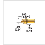
POGO-25H-S
