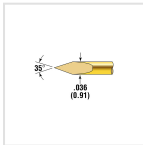
POGO-25T1-S
