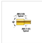
POGO-25I8-S
