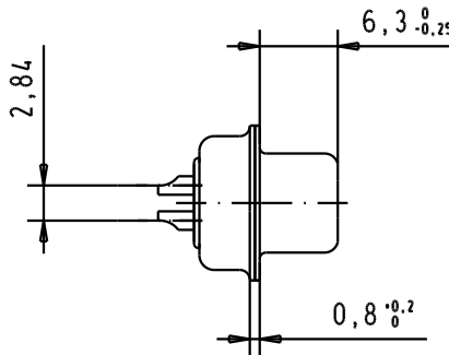
Solder bucket for AWG 20
