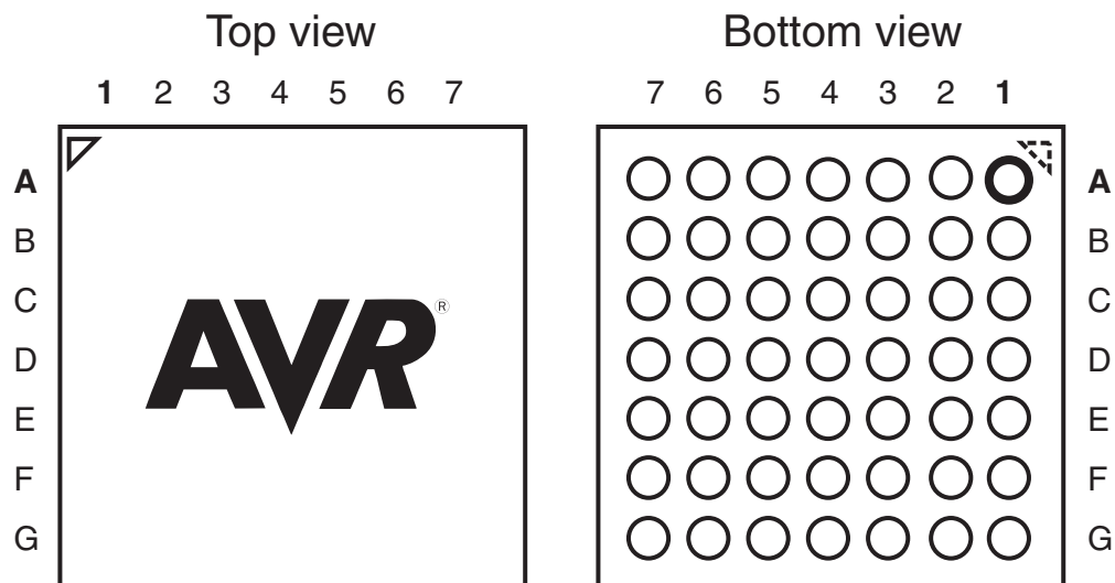
Figure 1-3. VFBGA - Pinout
