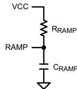
Figure 7-6. R_{RAMP} to VCC for V_{OUT} > 7.5 V
