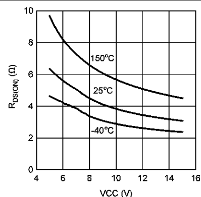
Figure 5-4. HO High R_{DS(ON)} vs VCC
