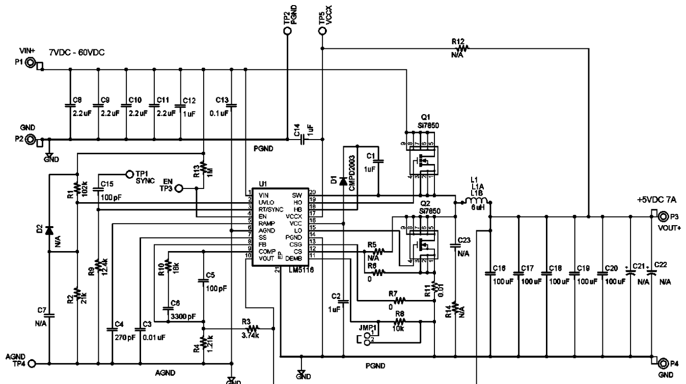
Figure 7-1. 5-V 7-A Typical Application Schematic
