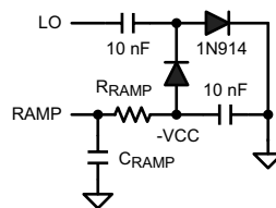
Figure 7-7. R_{RAMP} to -VCC for V_{OUT} < 7.5 V
