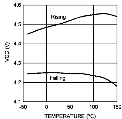
Figure 5-21. VCC UVLO vs Temperature
