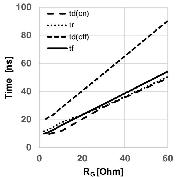
Figure 18 Typical switching times as a function of gate resistor (t = f(R_{G,ext}), V_{DD} = 800V, V_{GS} = 0V/18V, I_D = 13A, T_{vj} = 175^{\circ}C, \text{ind. load, test circuit} in Fig. E, diode: body diode at V_{GS} = 0V)
