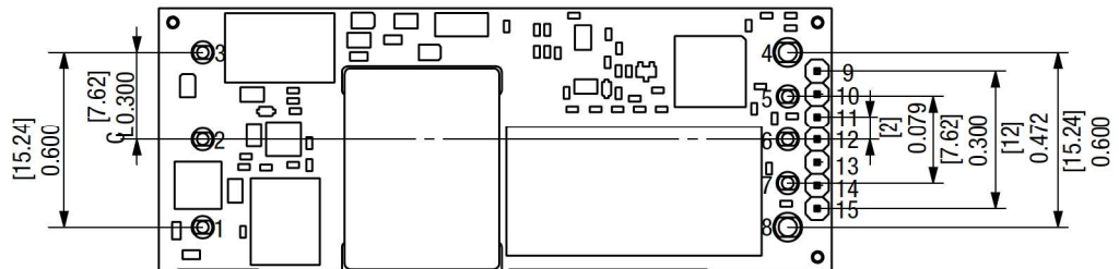
BOTTOM VIEW
