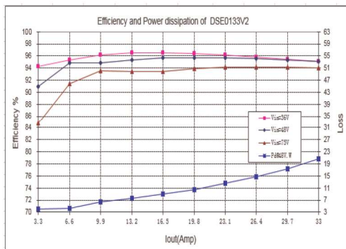
Figure 26. Efficiency and Power Dissipation
