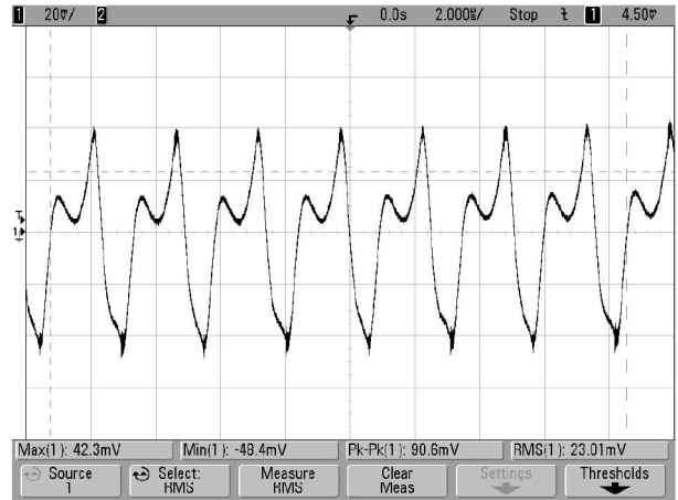
Figure 17. Ripple/Noise @+25°C (Vin=48V, Iout=33A, Cload=330µF, Scope BW=20MHz, 2µS/div, 20mV/div)
