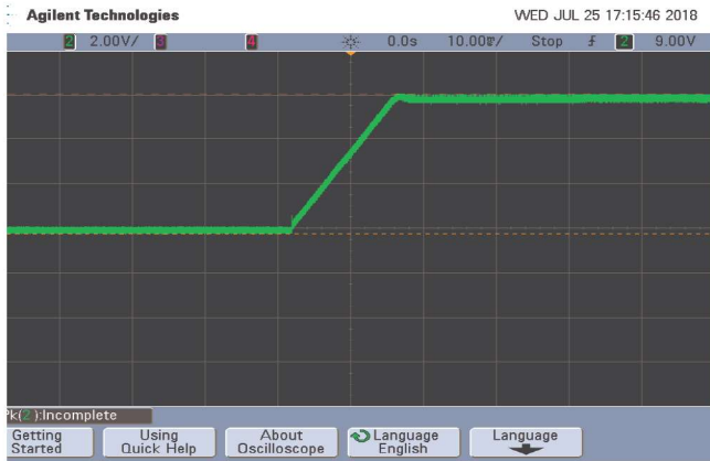
Figure 22. Output Pre-bias start-up Vin=48V, Iout = 0A, Cload = 47µF, Ta = 25°C, Pre-bias Voltage = 6V
