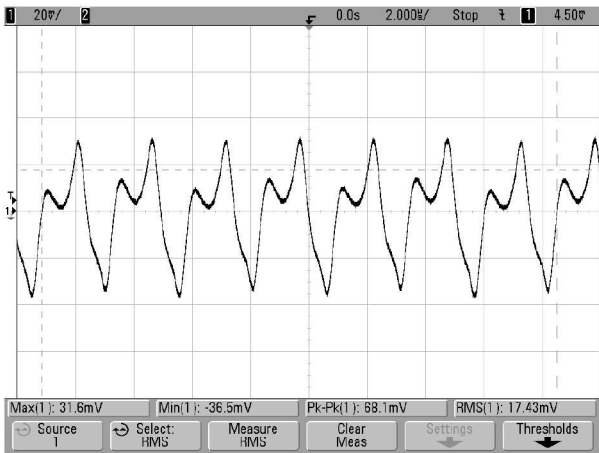
Figure 16. Ripple/Noise @+25°C (Vin=48V, Iout=0A, Cload=330µF, Scope BW=20MHz, 2µS/div, 20mV/div)
