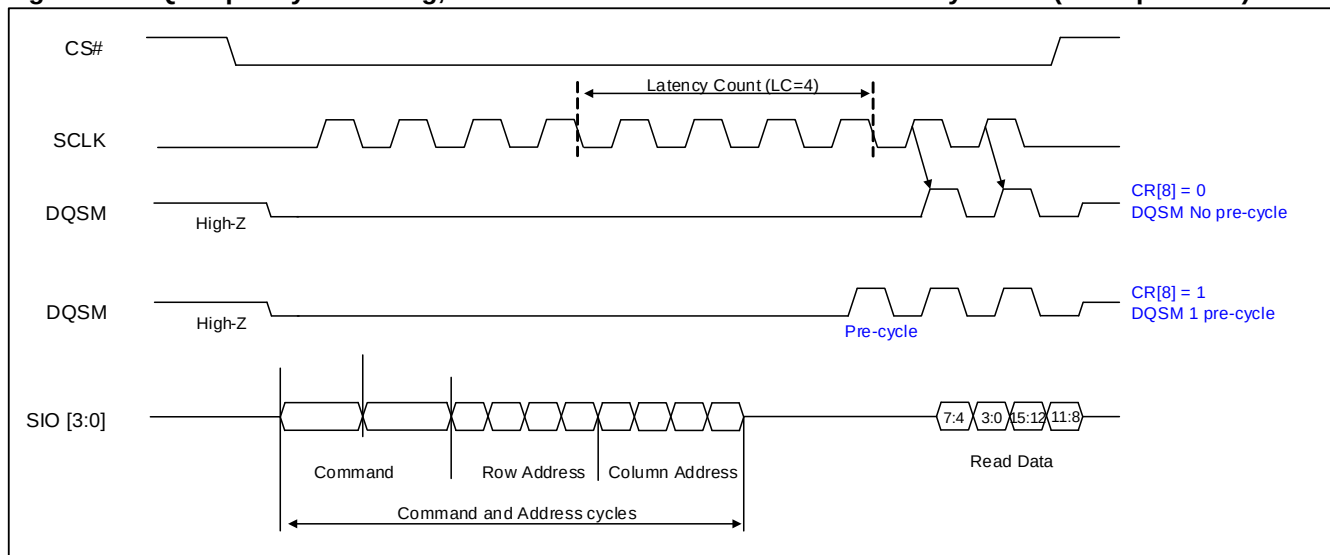
Figure 6.3 DQSM pre-cycle Timing, No Refresh Collision at Variable Latency READ (1LC operation)
