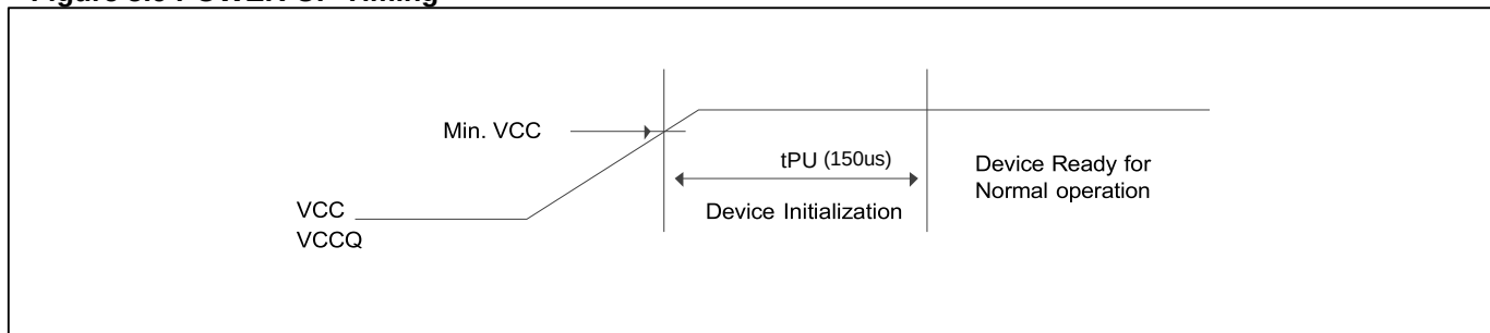
Figure 5.9 POWER-UP Timing
