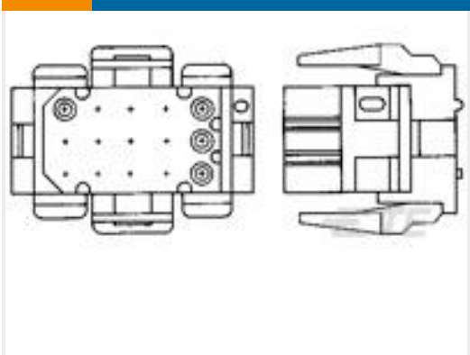
TE Part #1-640522-0 12P MR II PLUG HSG V0 RED
