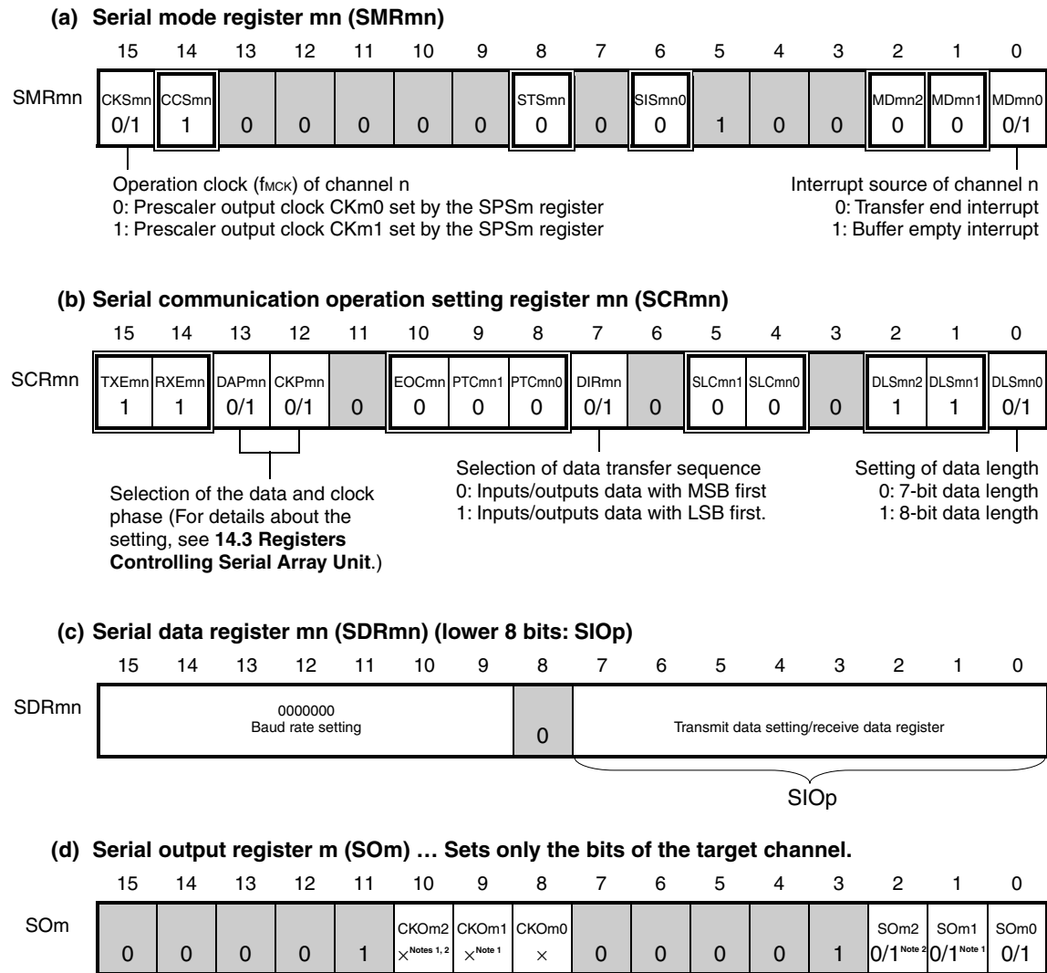
Figure 14-66. Example of Contents of Registers for Slave Transmission/Reception of 3-Wire Serial I/O (CSI00, CSI01, CSI10, CSI20, CSK40, CSK41) (1/2)
