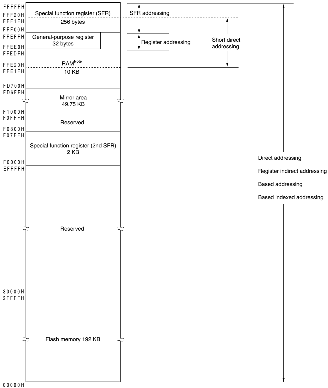
<R> Figure 4-18. Correspondence Between Data Memory and Addressing ( \mu PD78F1027, 78F1029)
