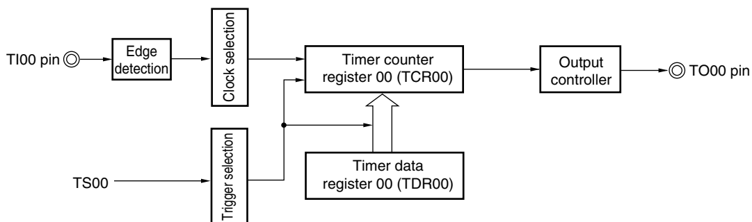
Figure 8-49. Block Diagram of Operation as Frequency Divider
