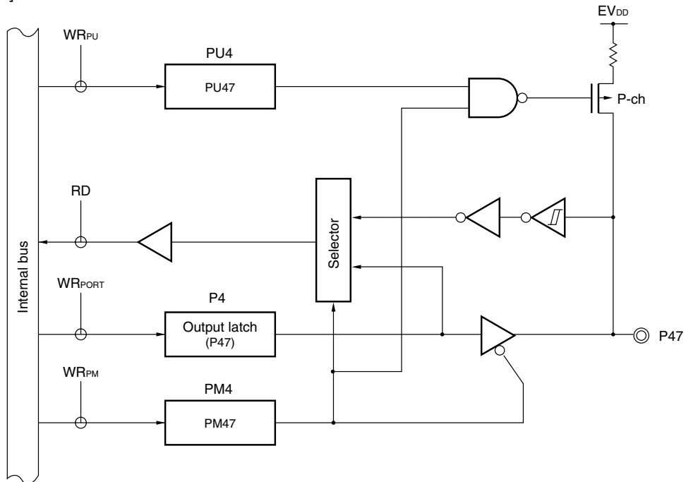
Figure 6-22. Block Diagram of P47
