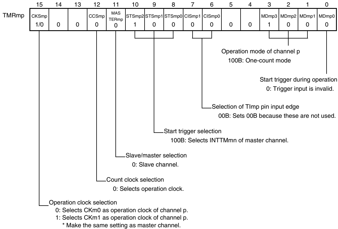
Figure 8-64. Example of Set Contents of Registers When One-Shot Pulse Output Function Is Used (Slave Channel)
