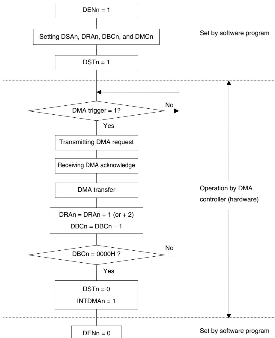
Figure 17-6. Operation Procedure
