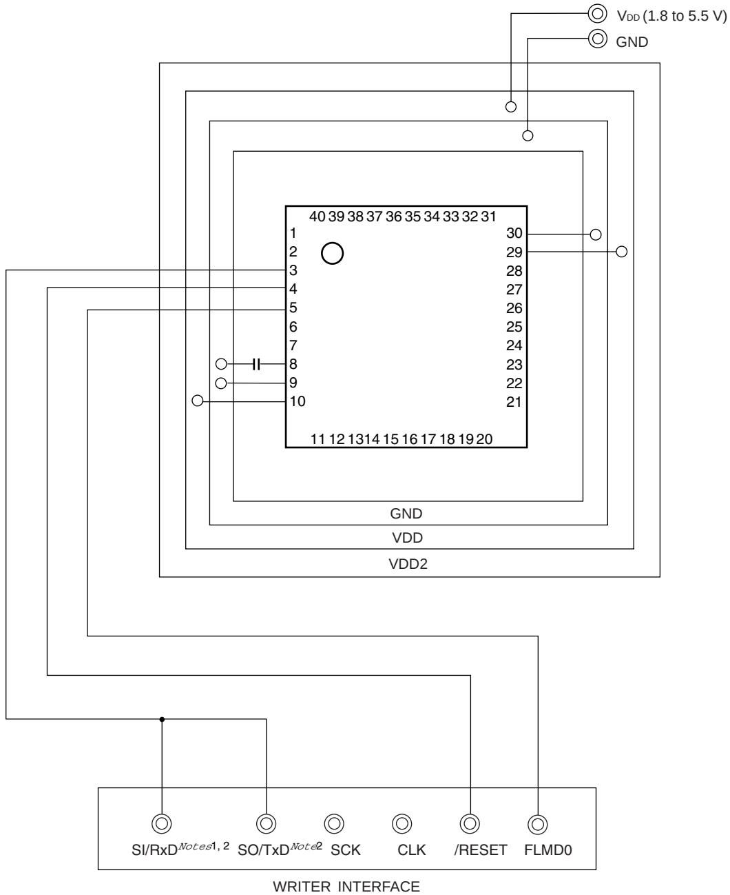
<R> Figure 26-1. Example of Wiring Adapter for Flash Memory Writing (40-pin product of 78K0R/KC3-L)
