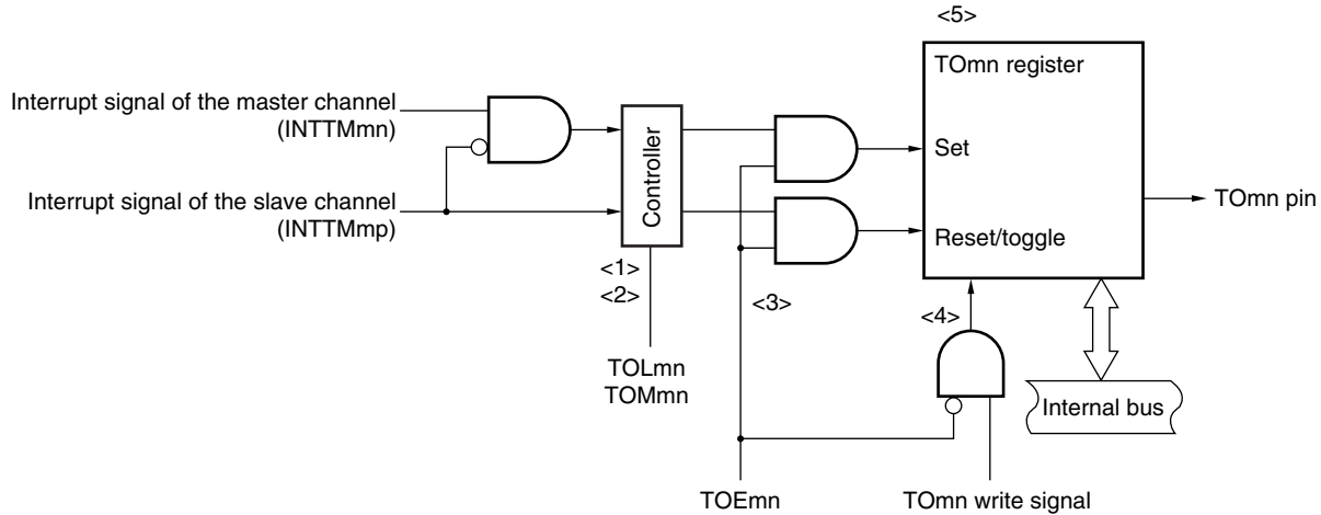
Figure 8-30. Output Circuit Configuration
