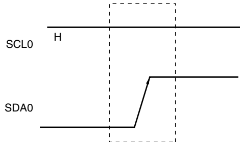
Figure 15-19. Stop Condition
