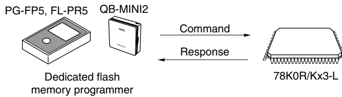
Figure 26-16. Communication Commands
