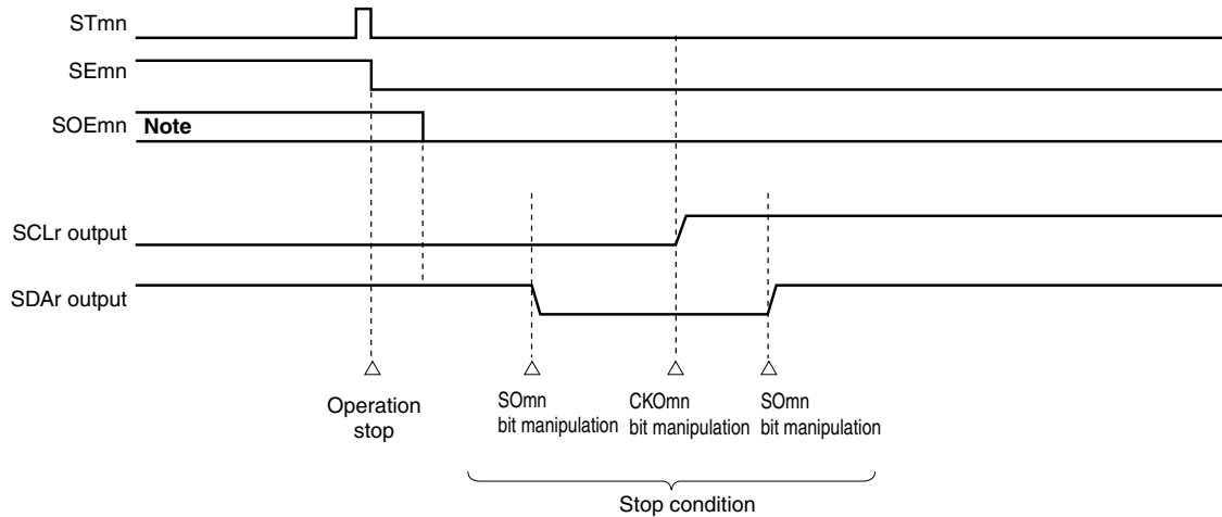
Figure 14-108. Timing Chart of Stop Condition Generation
