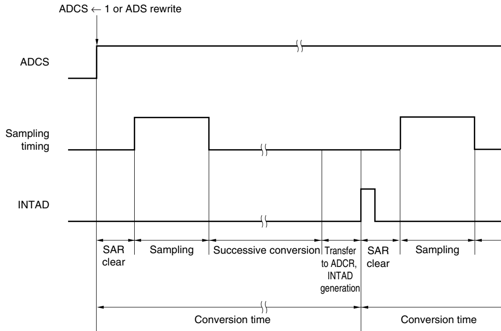
Figure 13-5. A/D Converter Sampling and A/D Conversion Timing
