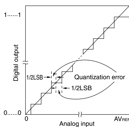
Figure 13-17. Quantization Error
