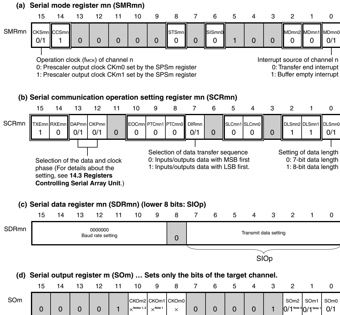
Figure 14-52. Example of Contents of Registers for Slave Transmission of 3-Wire Serial I/O (CSI00, CSI01, CSI10, CSI20, CSI40, CSI41) (1/2)
