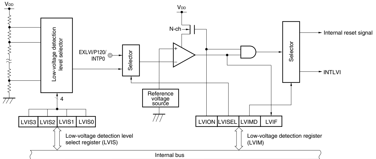
Figure 23-1. Block Diagram of Low-Voltage Detector
