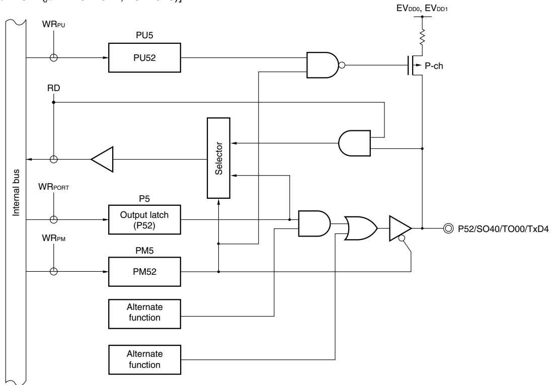
Figure 6-29. Block Diagram of P52
