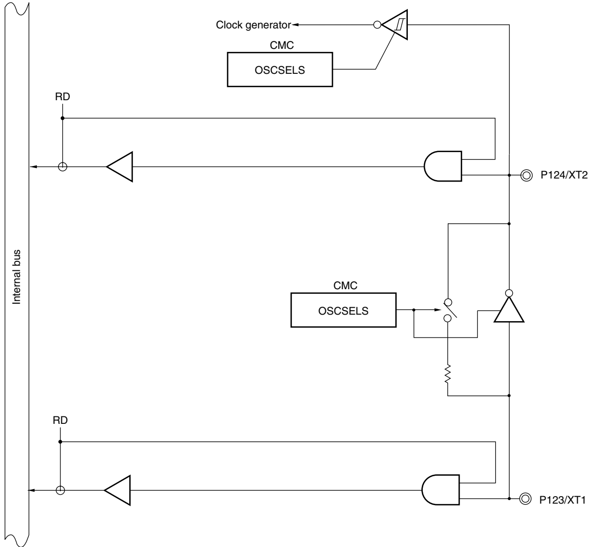
Figure 6-44. Block Diagram of P123 and P124
