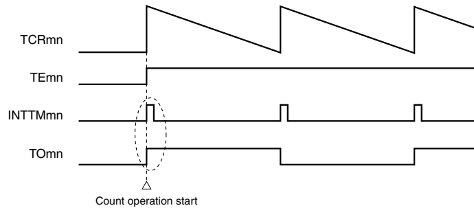
Figure 8-38. When MDmn0 is set to 1
