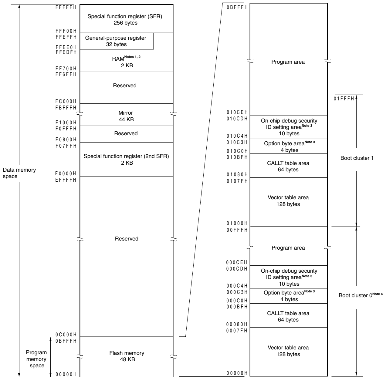
Figure 4-3. Memory Map ( \mu PD78F1002, 78F1005, 78F1008)
