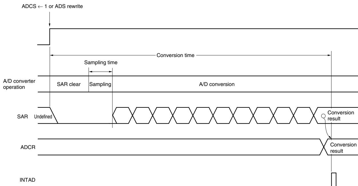
Figure 13-12. Basic Operation of A/D Converter
