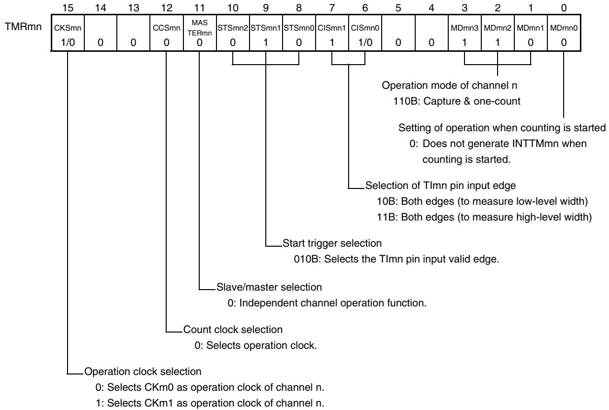
Figure 8-59. Example of Set Contents of Registers to Measure Input Signal High-/Low-Level Width
