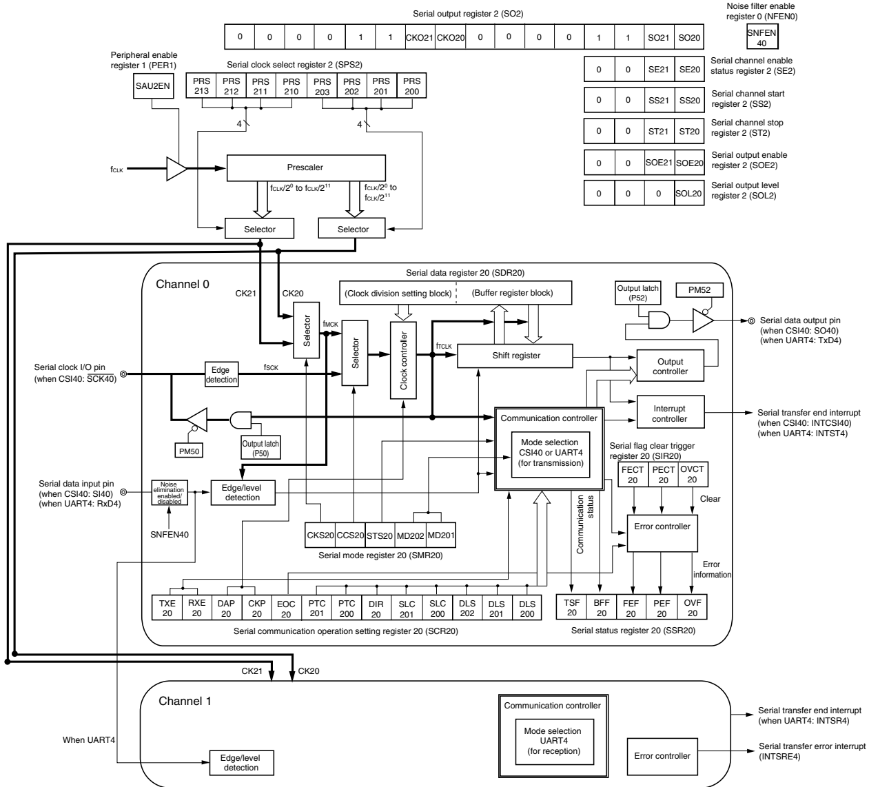
<R> Figure 14-3. Block Diagram of Serial Array Unit 1 (μ PD78F1027, 78F1028, 78F1029, 78F1030 only)
