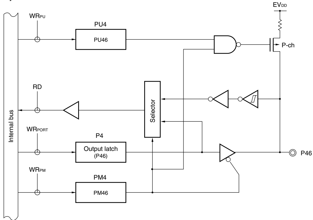
Figure 6-21. Block Diagram of P46
