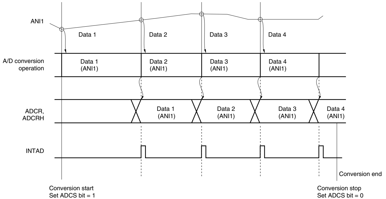
Figure 13-14. Example of Select Mode Operation Timing
