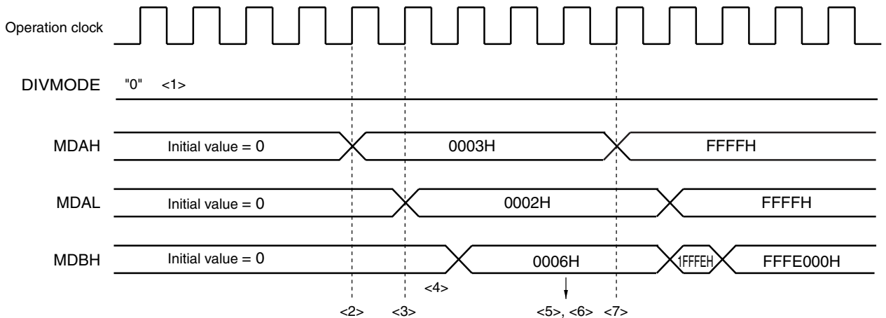
Figure 16-6. Timing Diagram of Multiplication Operation (0003H × 0002H)
