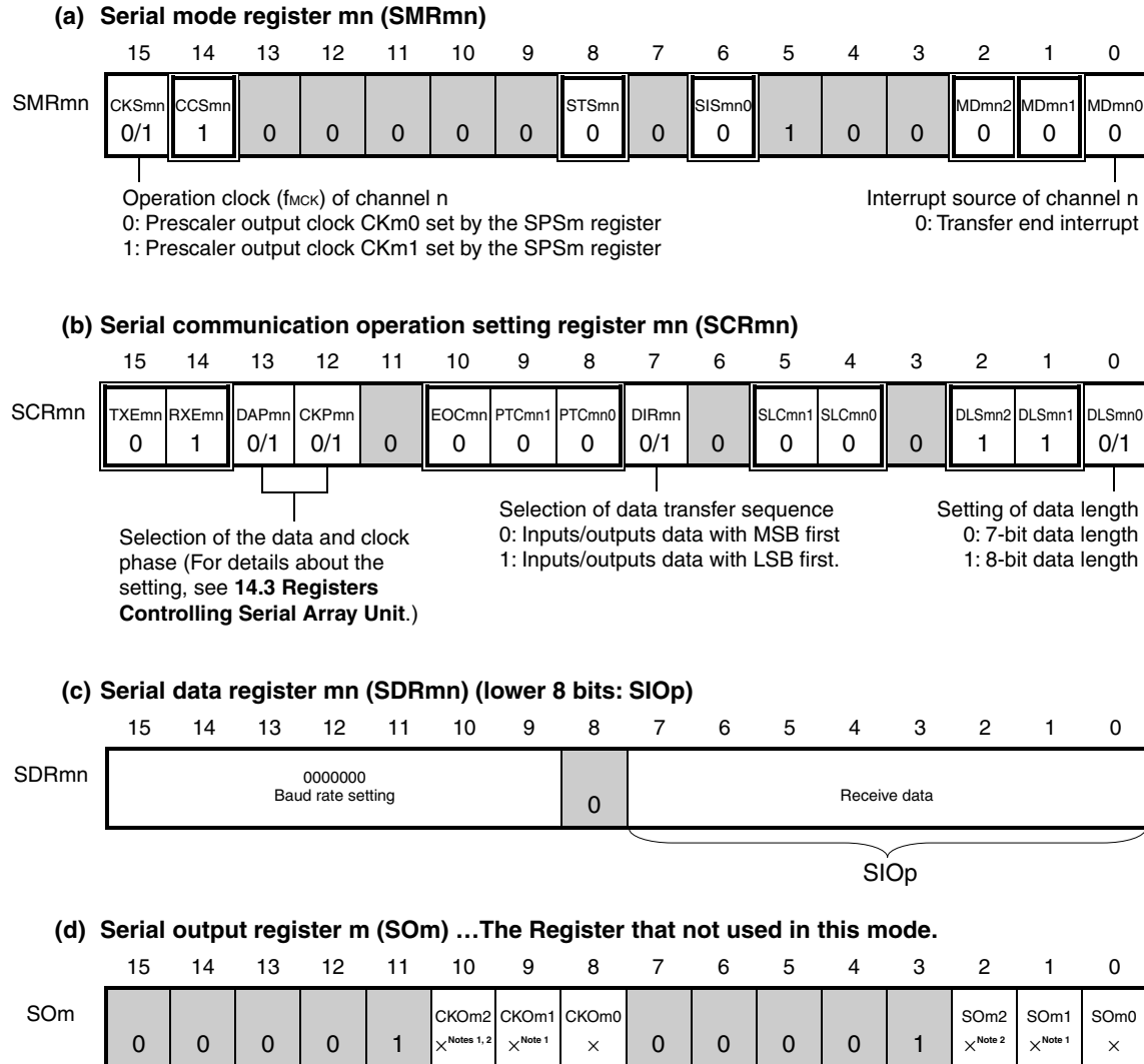
Figure 14-60. Example of Contents of Registers for Slave Reception of 3-Wire Serial I/O (CSI00, CSI01, CSI10, CSI20, CSI40, CSI41) (1/2)
