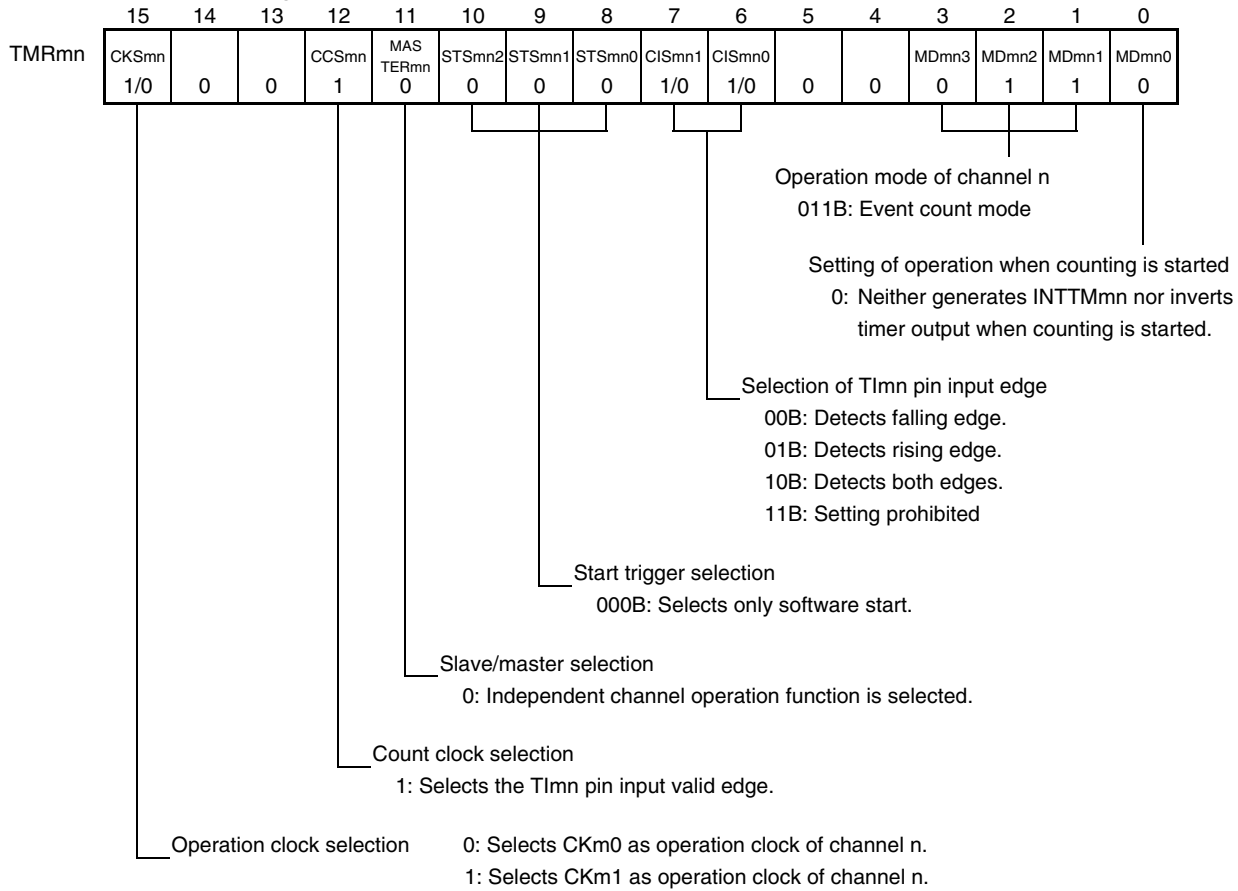
Figure 8-47. Example of Set Contents of Registers in External Event Counter Mode
