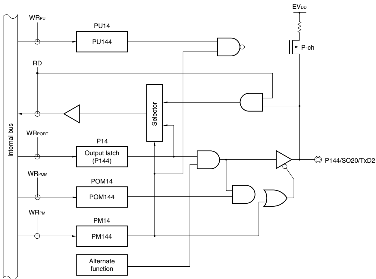
Figure 6-50. Block Diagram of P144
