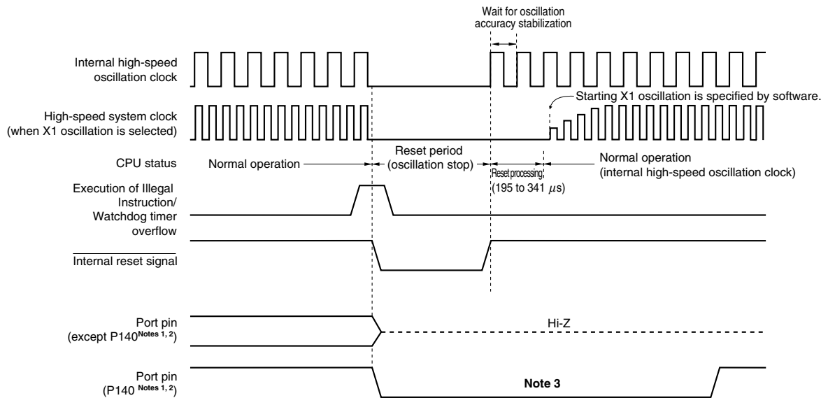
Figure 21-3. Timing of Reset Due to Execution of Illegal Instruction or Watchdog Timer Overflow
