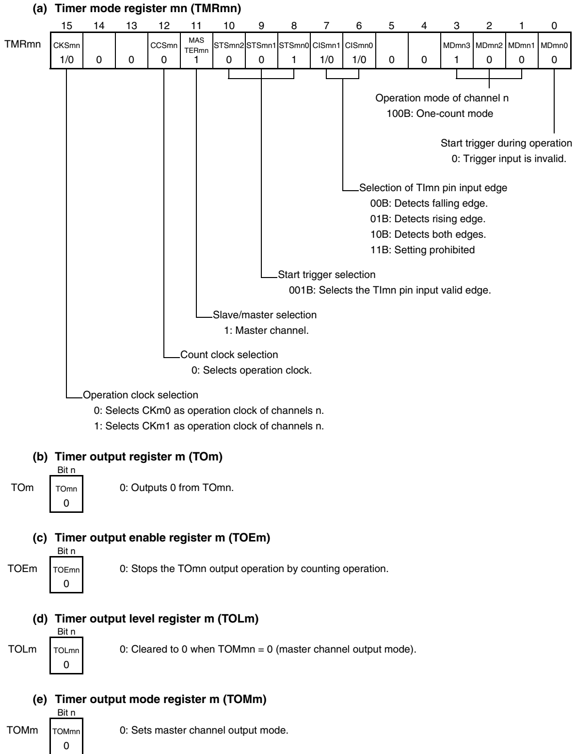
Figure 8-63. Example of Set Contents of Registers When One-Shot Pulse Output Function Is Used (Master Channel)
