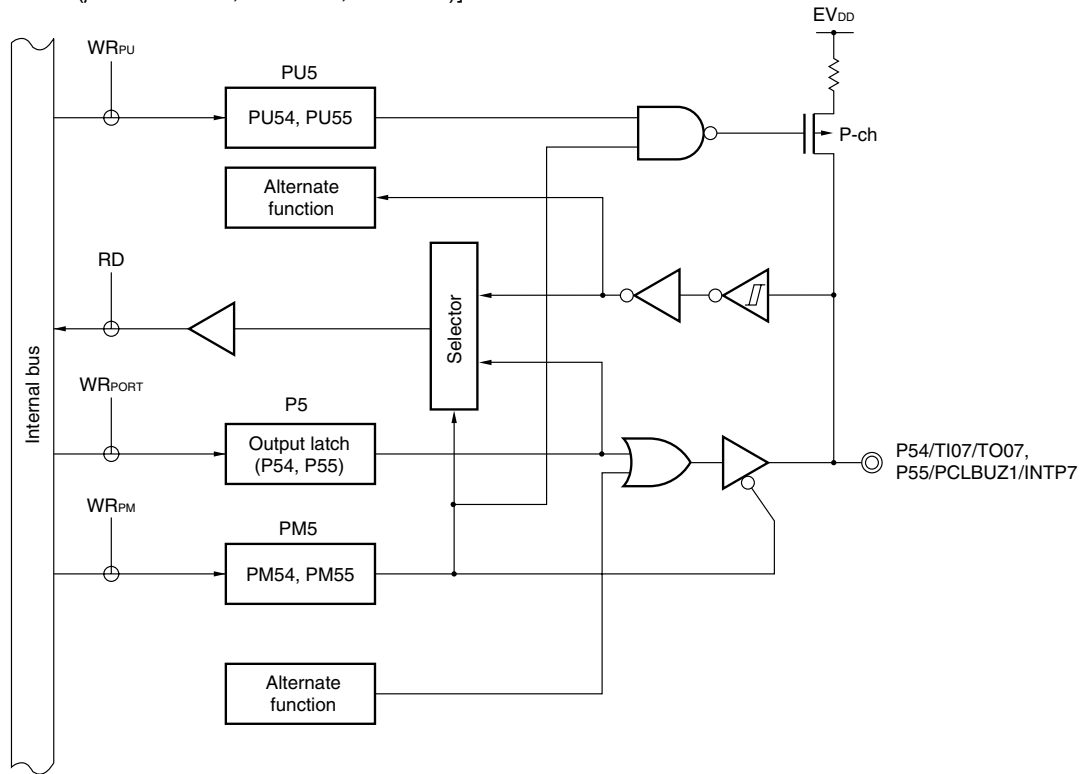
Figure 6-25. Block Diagram of P54 and P55
