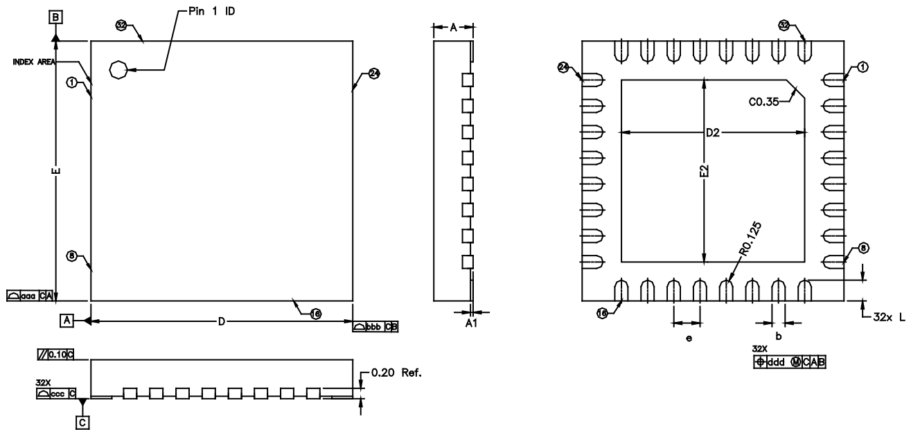
Figure 7.1. Package Drawing
