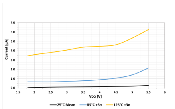
Figure 42-39. I PD Base
