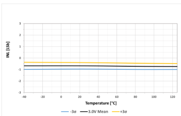
Figure 42-17. 8-BIT DAC, INL vs. Temperature ( V_{REF} = V_{DD} = 3.0V )
