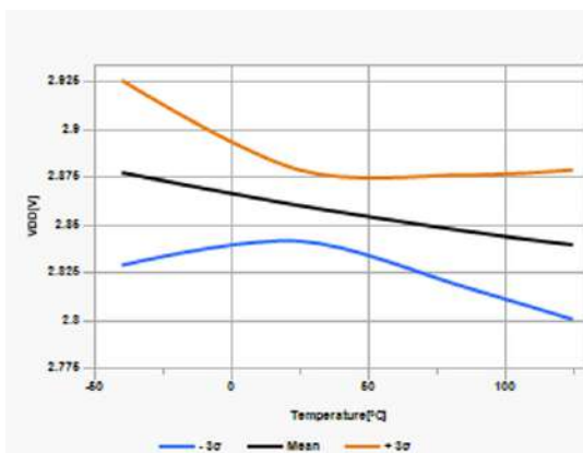
Figure 42-7. Brown-out Reset Voltage, Trip Point (BORV = 0)
