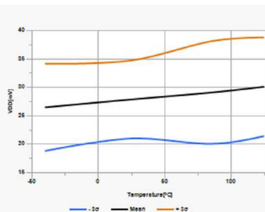
Figure 42-8. Brown-out Reset Hysteresis, Trip Point (BORV = 0)
