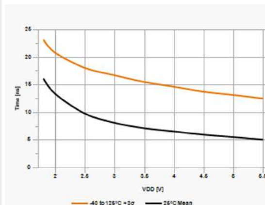
Figure 42-31. Fall Time, Slew Rate Control Disabled
