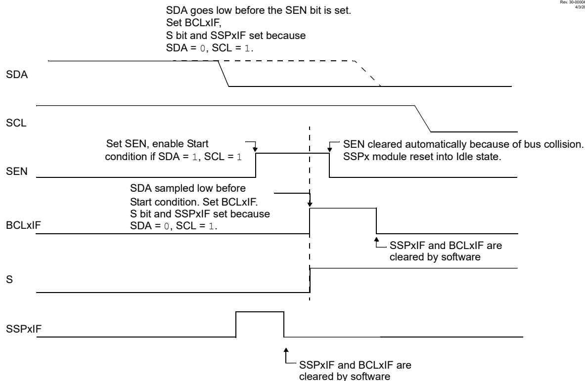
Figure 29-34. Bus Collision During Start Condition (SDA Only)
