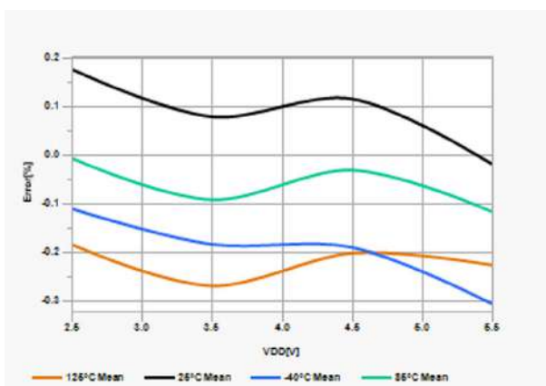
Figure 42-22. FVR Voltage Error vs. V_{DD} 2x ( V_{REF} = 2.048V )
