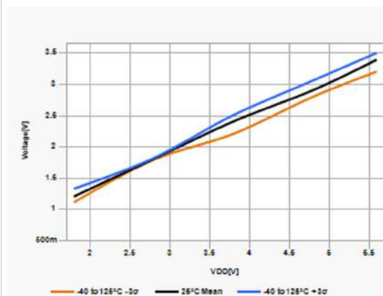
Figure 42-34. Schmitt Trigger High Values (V IH vs. V DD )
