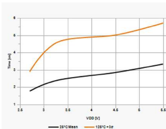
Figure 42-11. BOR Response Time
