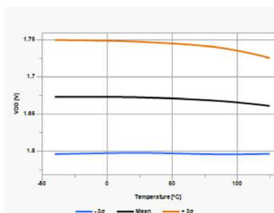
Figure 42-50. POR Release Voltage
