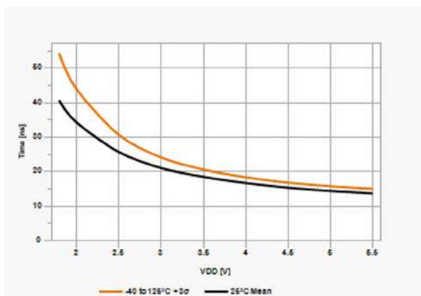
Figure 42-29. Fall Time, Slew Rate Control Enabled
