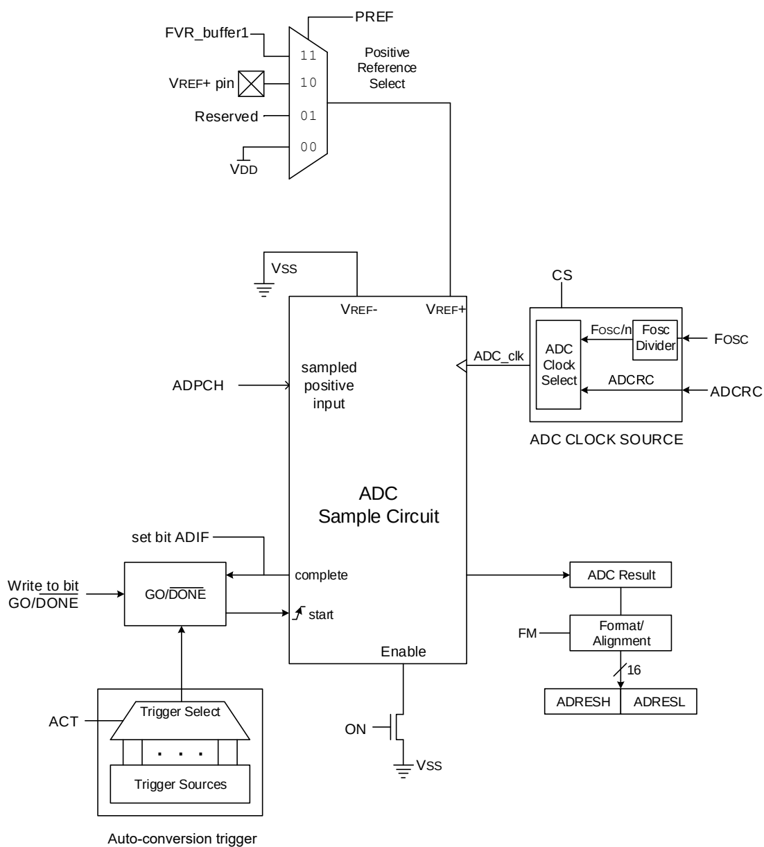
Figure 31-1. ADC Block Diagram
