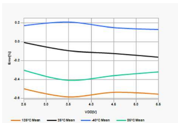
Figure 42-21. FVR Voltage Error vs. V_{DD} 1x ( V_{REF} = 1.024V )
