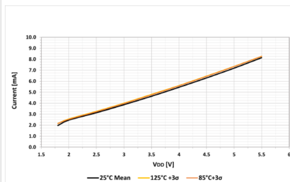
Figure 42-33. I DD , HFINTOSC, F HFO = 32 MHz
