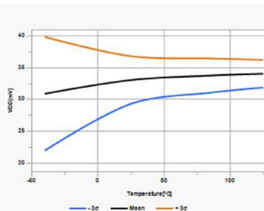
Figure 42-10. Brown-out Reset Hysteresis, Trip Point (BORV = 1)
