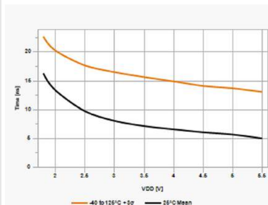
Figure 42-30. Rise Time, Slew Rate Control Disabled
