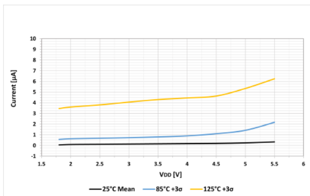
Figure 42-40. I PD ADC (ADC is non-converting)
