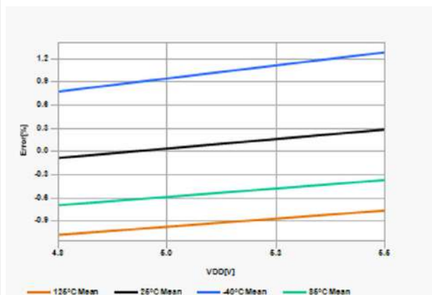
Figure 42-23. FVR Voltage Error vs. V_{DD} 4x ( V_{REF} = 4.096V )
