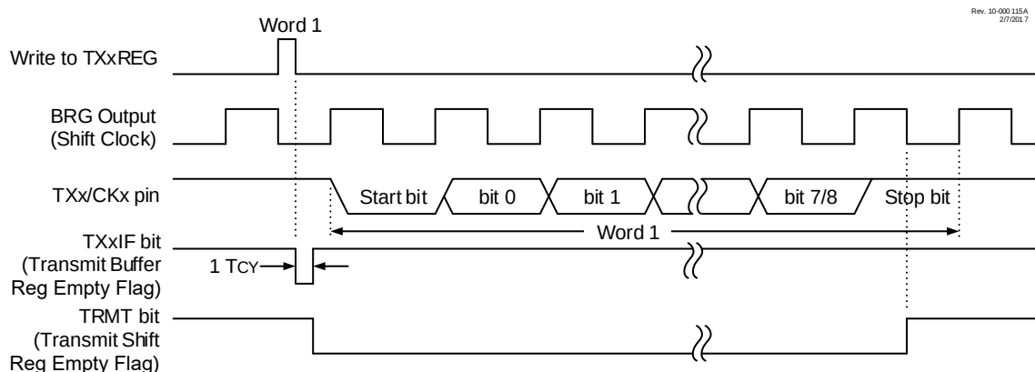
Figure 30-3. Asynchronous Transmission
