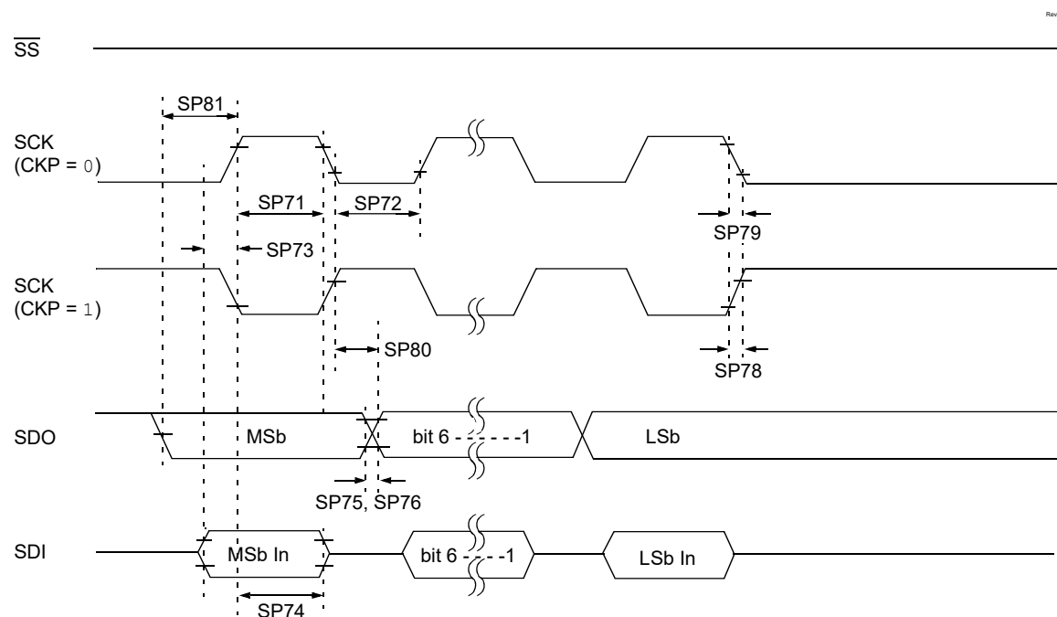
Figure 41-16. SPI Host Mode Timing (CKE = 1, SMP = 1)
