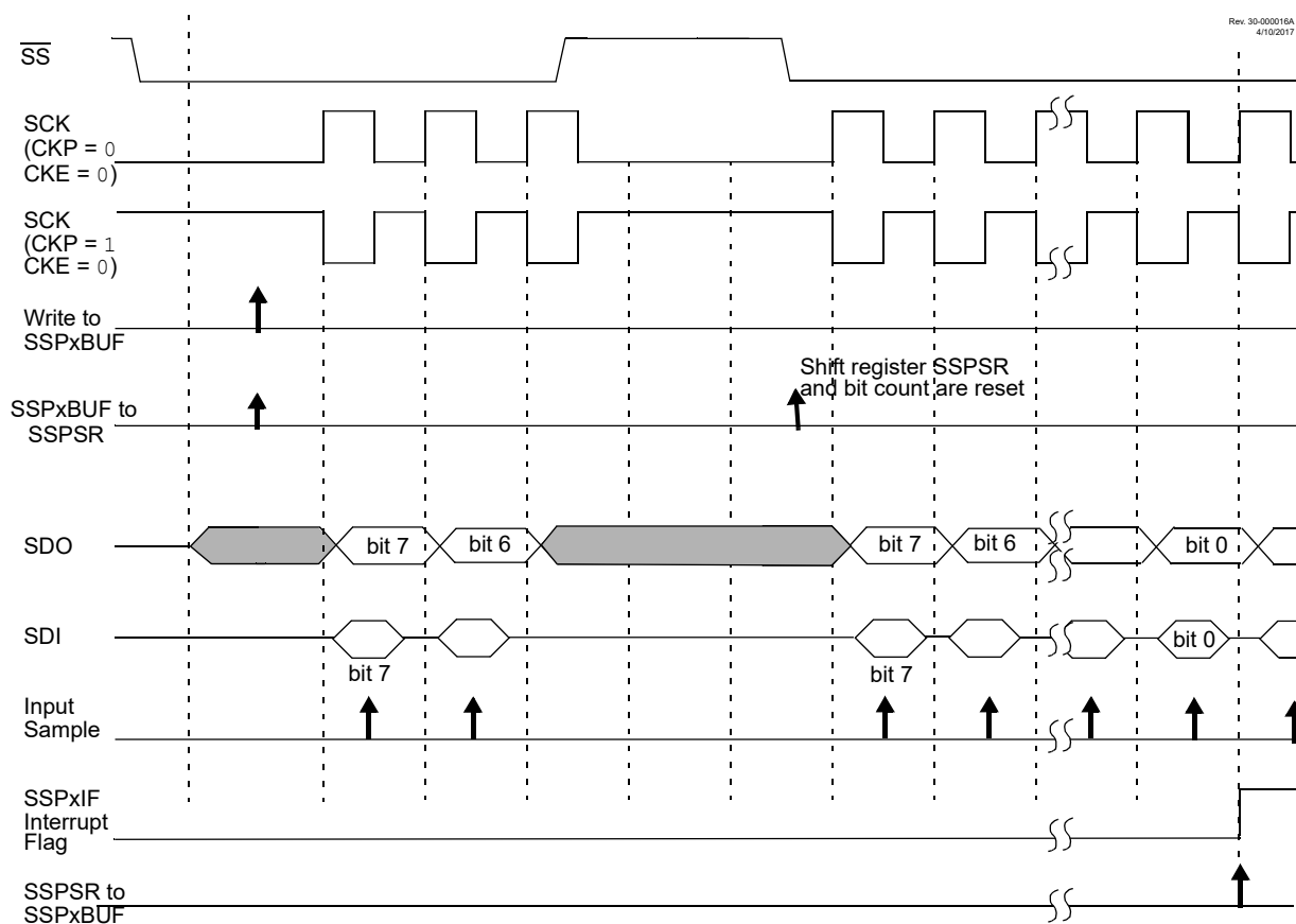
Figure 29-6. Client Select Synchronous Waveform
