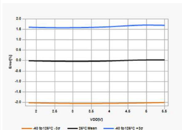
Figure 42-25. HFINTOSC Error % over V_{DD}
