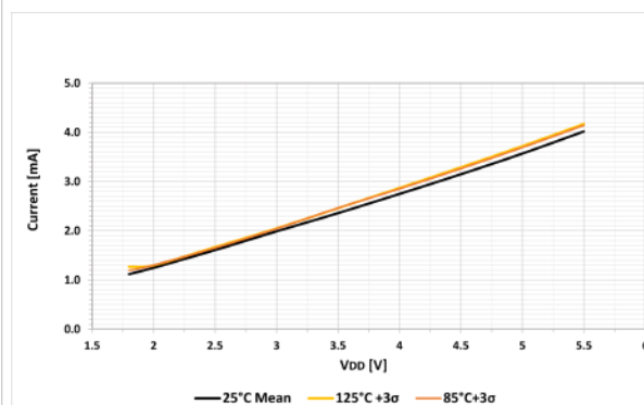
Figure 42-32. I DD , HFINTOSC, F HFO = 16 MHz
