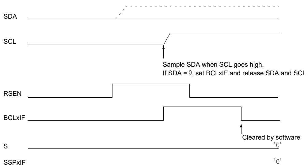
Figure 29-37. Bus Collision During a Repeated Start Condition (Case 1)
