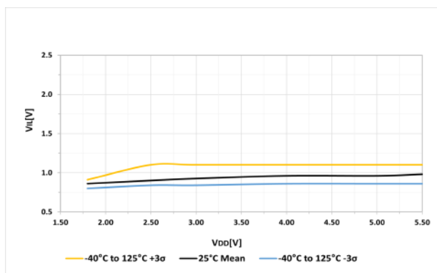
Figure 42-38. SMBus 3.0 Low Value (V IL vs. V DD )
