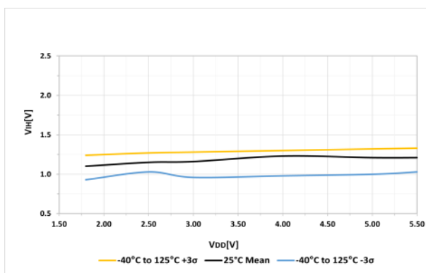
Figure 42-37. SMBus 3.0 High Value (V IH vs. V DD )
