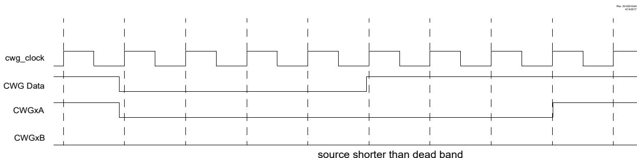
Figure 23-13. Dead-Band Operation, CWGxDBR = 0 \times 03 , CWGxDBF = 0 \times 06 , Source Shorter Than Dead Band
