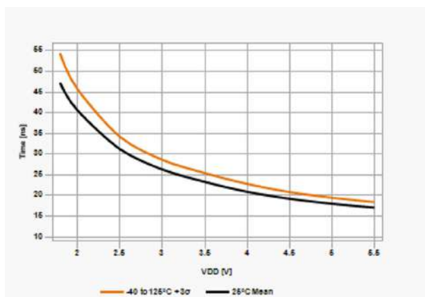
Figure 42-28. Rise Time, Slew Rate Control Enabled
