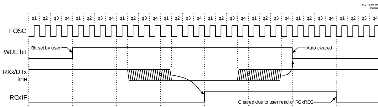
Figure 30-7. Auto-Wake-Up (WUE) Bit Timing During Normal Operation
