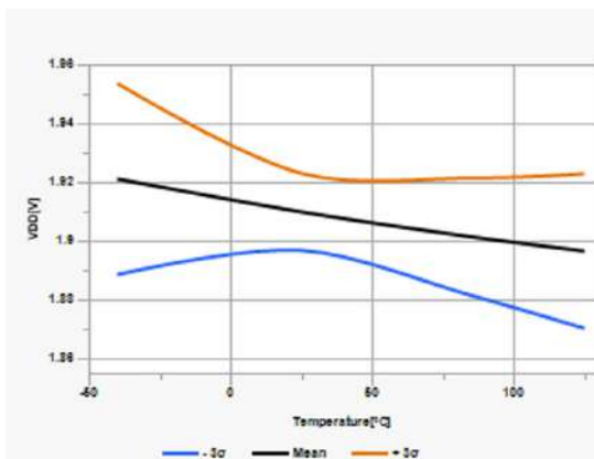
Figure 42-9. Brown-out Reset Voltage, Trip Point (BORV = 1)
