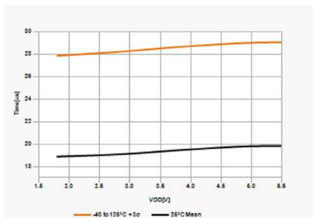
Figure 42-27. Wake From Sleep, HFINTOSC = 4 MHz
