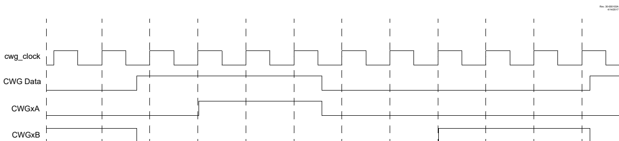
Figure 23-12. Dead-Band Operation, CWGxDBR = 0 \times 01 , CWGxDBF = 0 \times 02
