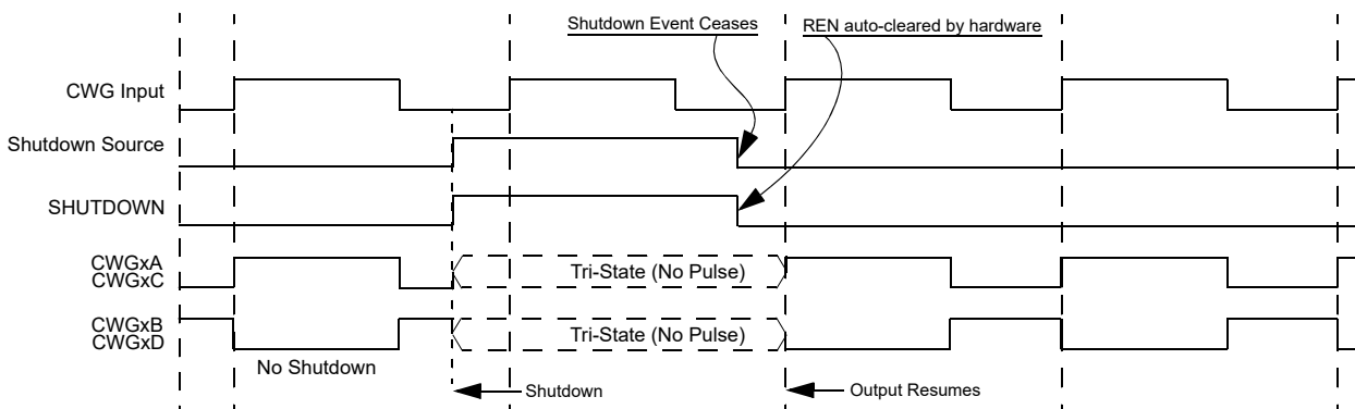
Figure 23-16. Shutdown Functionality, Auto-Restart Enabled (REN = 1, LSAC = 'b01, LSBD = 'b01)
