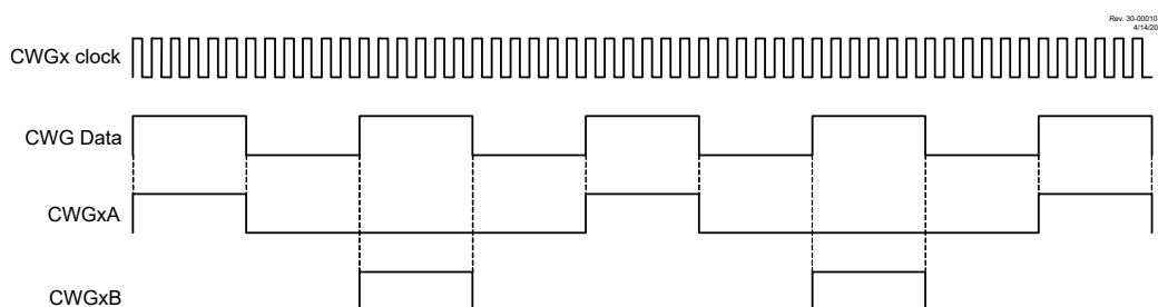
Figure 23-10. Example of Synchronous Steering (MODE = 'b001)
