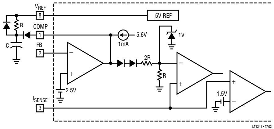
Soft-Start
