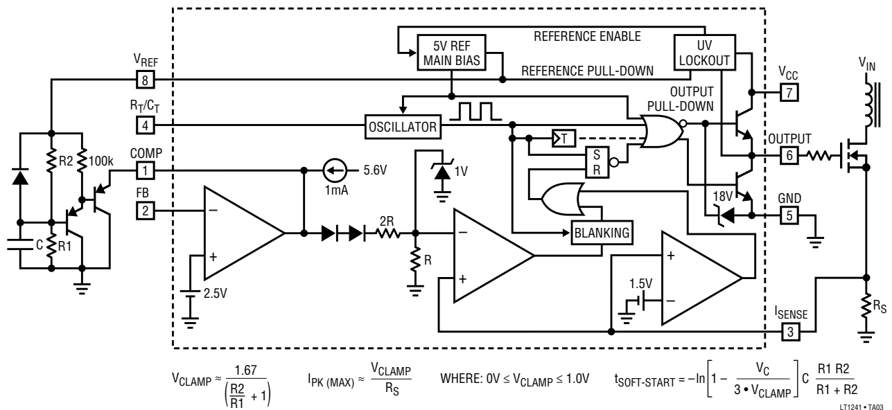
Adjustable Clamp Level with Soft-Start
