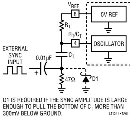
External Clock Synchronization
